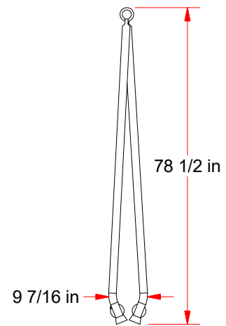
STORAGE VIEW
